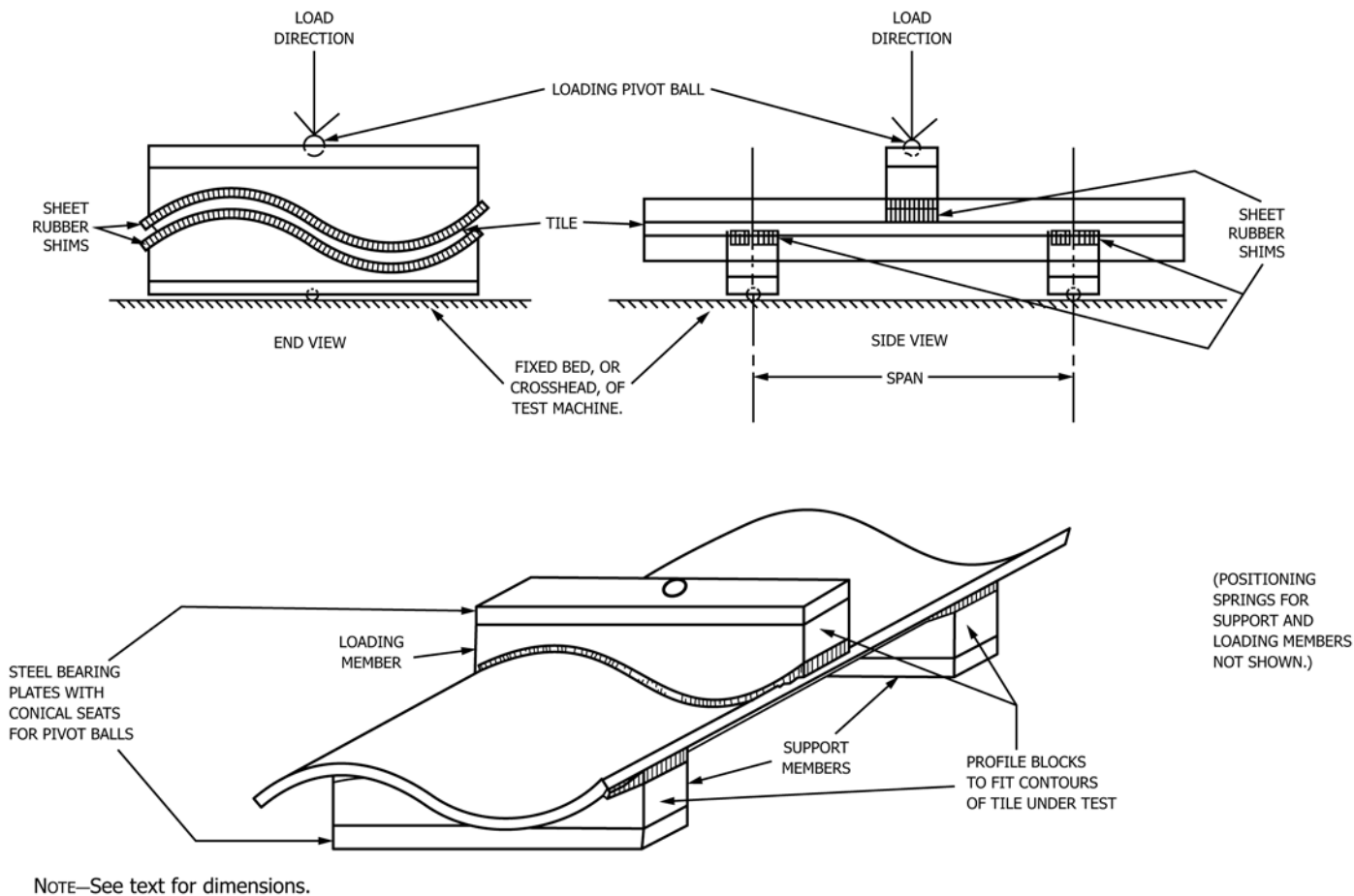
FIG. 1 Schematic of Assembly for Flexure Strength Testing
